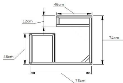
Gambar 2 Tampak Samping
